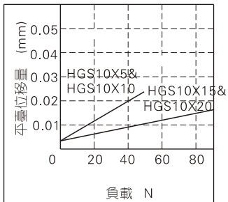
HGS10 L=100mm
