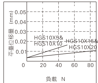
HGS10 L=100mm
