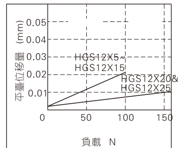
HGS12 L=100mm
